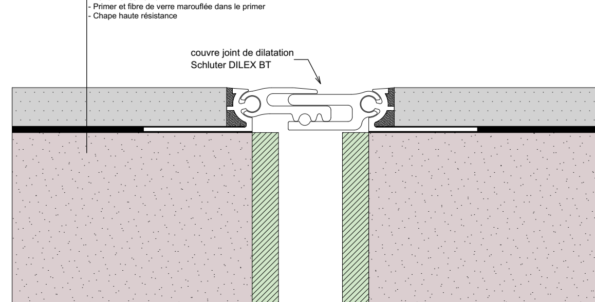
JOINT DE DILATATION STRUCTUREL
